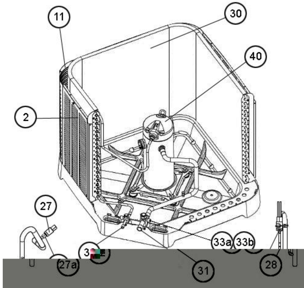
Valve Mounting, Compressor
